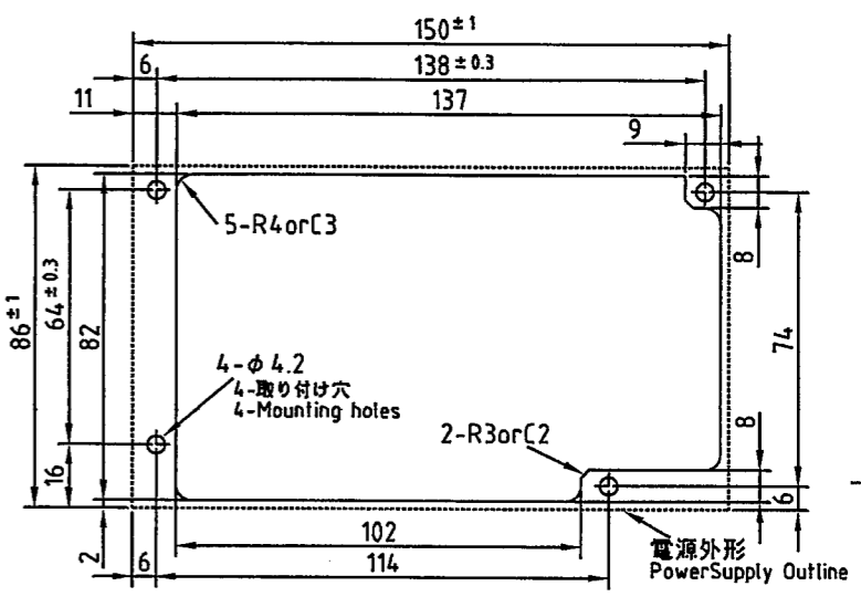
推奨電源取り付け穴加工図 Recommended a installation hole and 4 mounting holes
