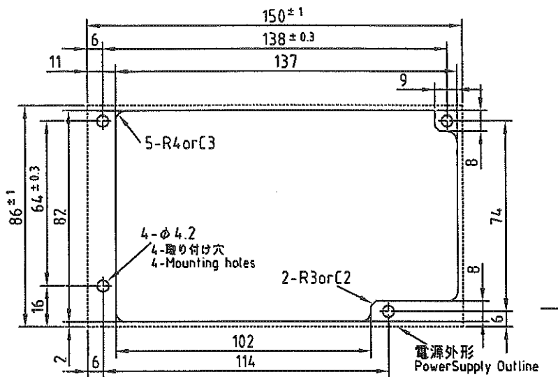
推奨電源取り付け穴加工図 Recommended a installation hole and 4 mounting holes
